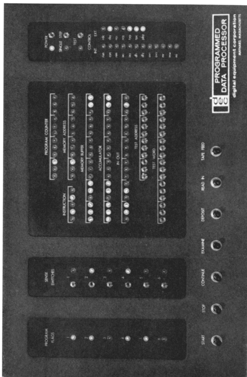
PDP-1 CONTROL PANEL
