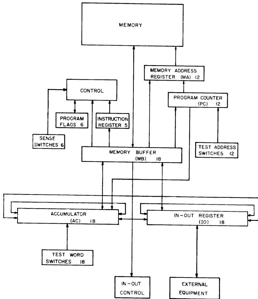
PDP-1 SYSTEM BLOCK DIAGRAM
